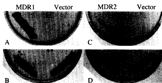
Fig. 2. Resistance of S. cerevisiae W303-1AY18 harboring human MDR1 or MDR2 expression vector. Over-night cultures of W303-1AY18 harboring the control vector, pYM/ MDR1 or pYM/ MDR2 were diluted to A_{595} = 1.0 by media and streaked on SD plates containing 0 (B and D), 0.1 (C), or 0.15 \mu\text{g/ml} aureobasidin A (A). The plates were incubated at 30°C for 3 days.
