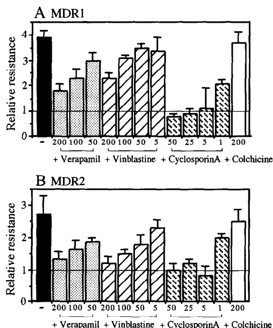
Fig. 5. Effects of MDR modulators on aureobasidin A resistance of W303-1AY18 harboring pYM/MDR1 (A) or pYM/MDR2 (B). Growth inhibition assay was done in the absence (–) or in the presence of verapamil (50, 100, and 200 \mu M), vinblastine (5, 50, 100, and 200 \mu M), cyclosporin A (1, 5, 25, and 50 \mu M), or colchicine (200 \mu M) as described in Section 2. The results are presented relative to W303-1AY18 harboring the control vector. MDR modulators of these concentrations have no effect on the growth of W303-1AY18. Each bar represents the average of at least three experiments.
