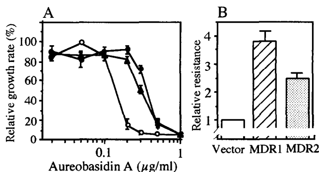
Fig. 3. A: Growth inhibition assay of W303-1AY18 harboring the control vector ( \circ ), pYM/ MDR1 ( \bullet ) or pYM/ MDR2 ( \blacktriangle ). The assay was done in triplicate as described in Section 2. The values are expressed relative to each transformant strain grown in the absence of the drug. B: Relative resistance of W303-1AY18 harboring the control vector, pYM/ MDR1 or pYM/ MDR2 . Relative resistance was calculated by comparing the \text{IC}_{50} s. The results are presented relative to W303-1AY18 harboring the control vector. Each bar represents the average of three experiments.
