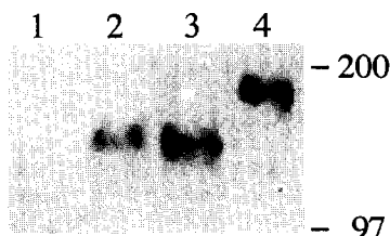
Fig. 1. Immunoblotting of membrane fraction from S. cerevisiae W303-1AY18/vector (lane 1), W303-1AY18/ MDR1 (lane 2), W303-1AY18/ MDR2 (lane 3) and human MDR1 cultured cells KB-G2 [10] (lane 4). 20 \mu\text{g} of membrane protein was put on each lane, and was reacted with monoclonal antibody C219 as a probe for P-glycoprotein. Molecular size standards are indicated in kDa on the right.
